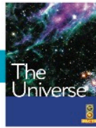
The Universe
