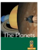
The Planets
