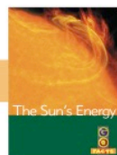
The Sun's Energy
