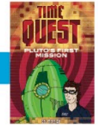
Pluto's First Mission
