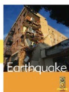
Earthquake
