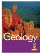
Geology
