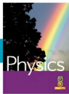
Physics
