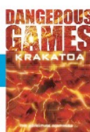
Krakatoa
