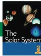
The Solar System
